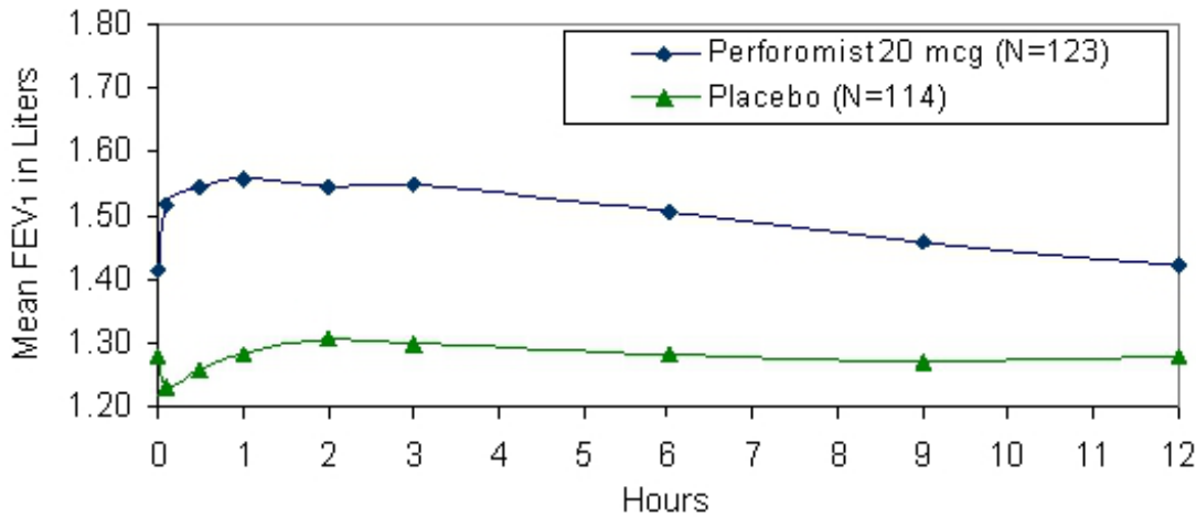
Figure 1 Mean* FEV1 at Day 1
