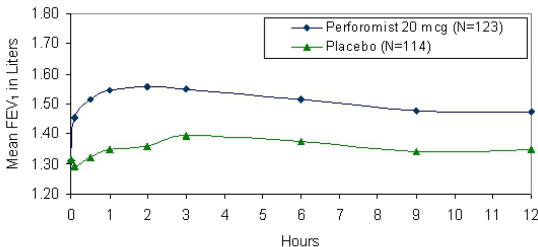
Figure 1 Mean* FEV1 at Day 1
